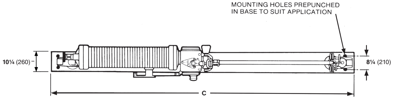
POLE-UNIT TOP VIEW
