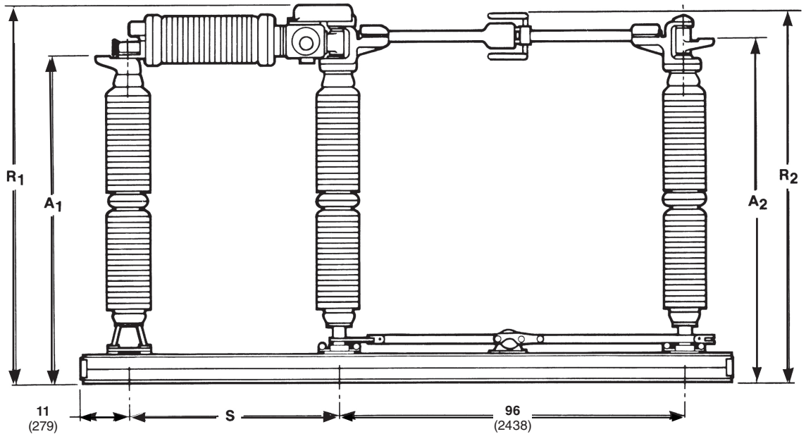
POLE-UNIT SIDE VIEW
