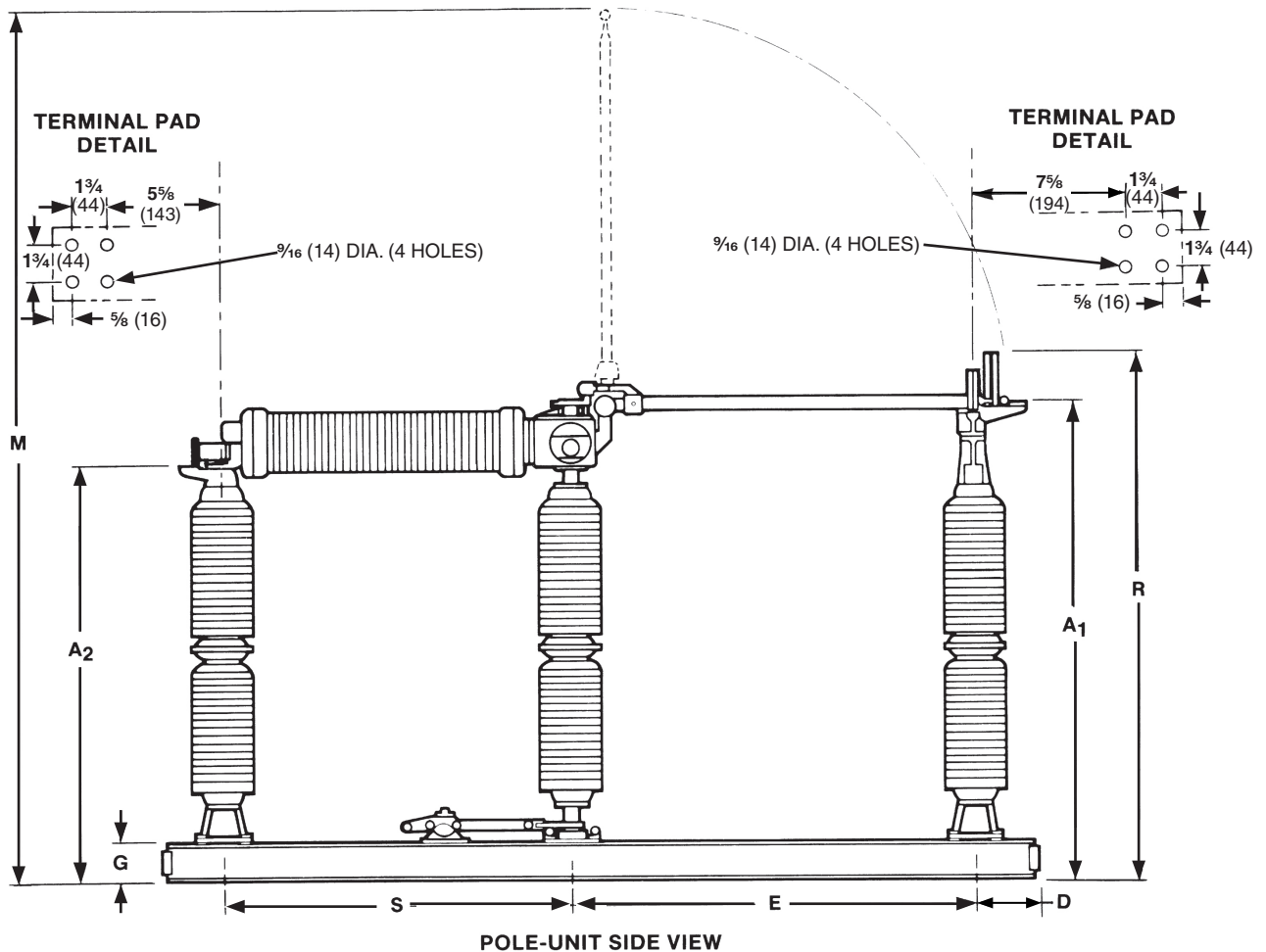
POLE-UNIT SIDE VIEW
