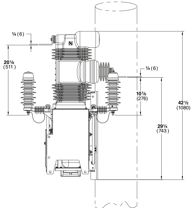
SIDE VIEW
